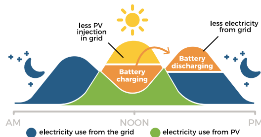
Figure 3. Peak load shifting using a battery. (Source: SCM Solution Booklet PV and Battery )
